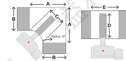
3M Keyboard Tray Installation Minimums: 3M 鍵盤托安裝最低要求
